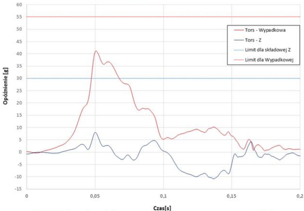
Graph 6. Decelerations of the chest for 32 kg dummy during dynamic test - variant 2
