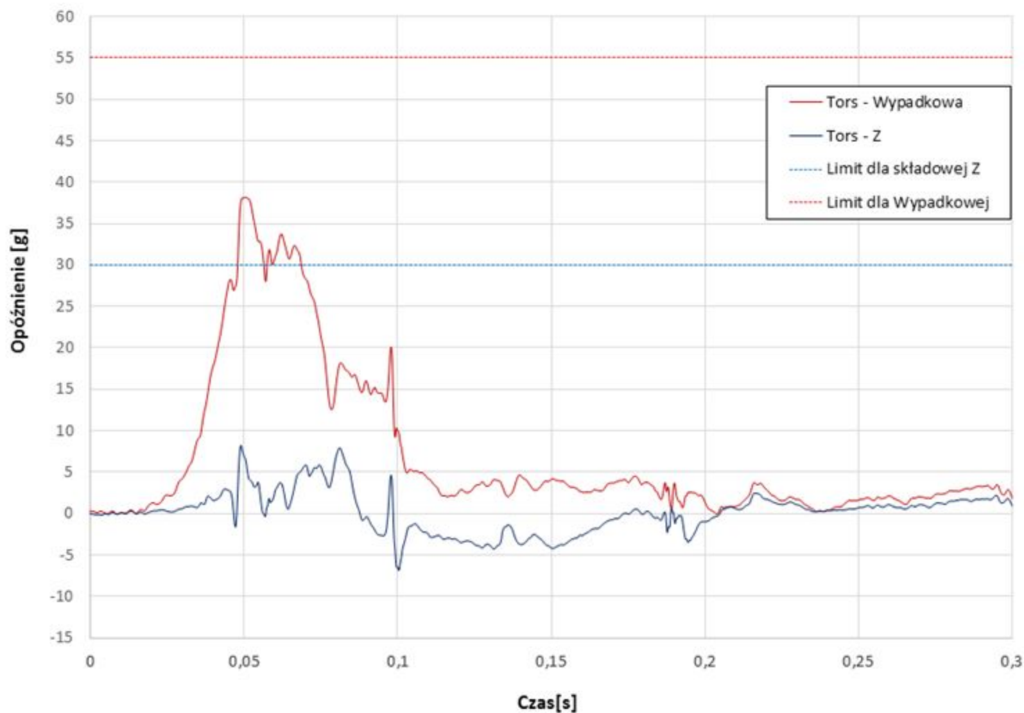
Graph 2. Decelerations of the chest for 15 kg dummy during dynamic test - variant 1
