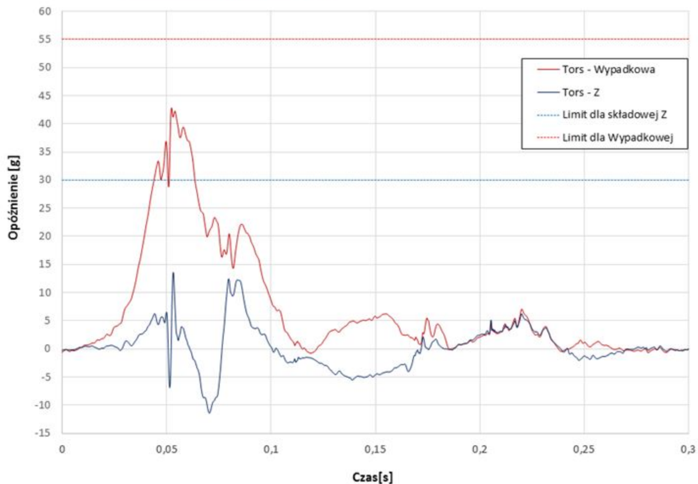
Graph 5. Decelerations of the chest for 15 kg dummy during dynamic test - variant 2
