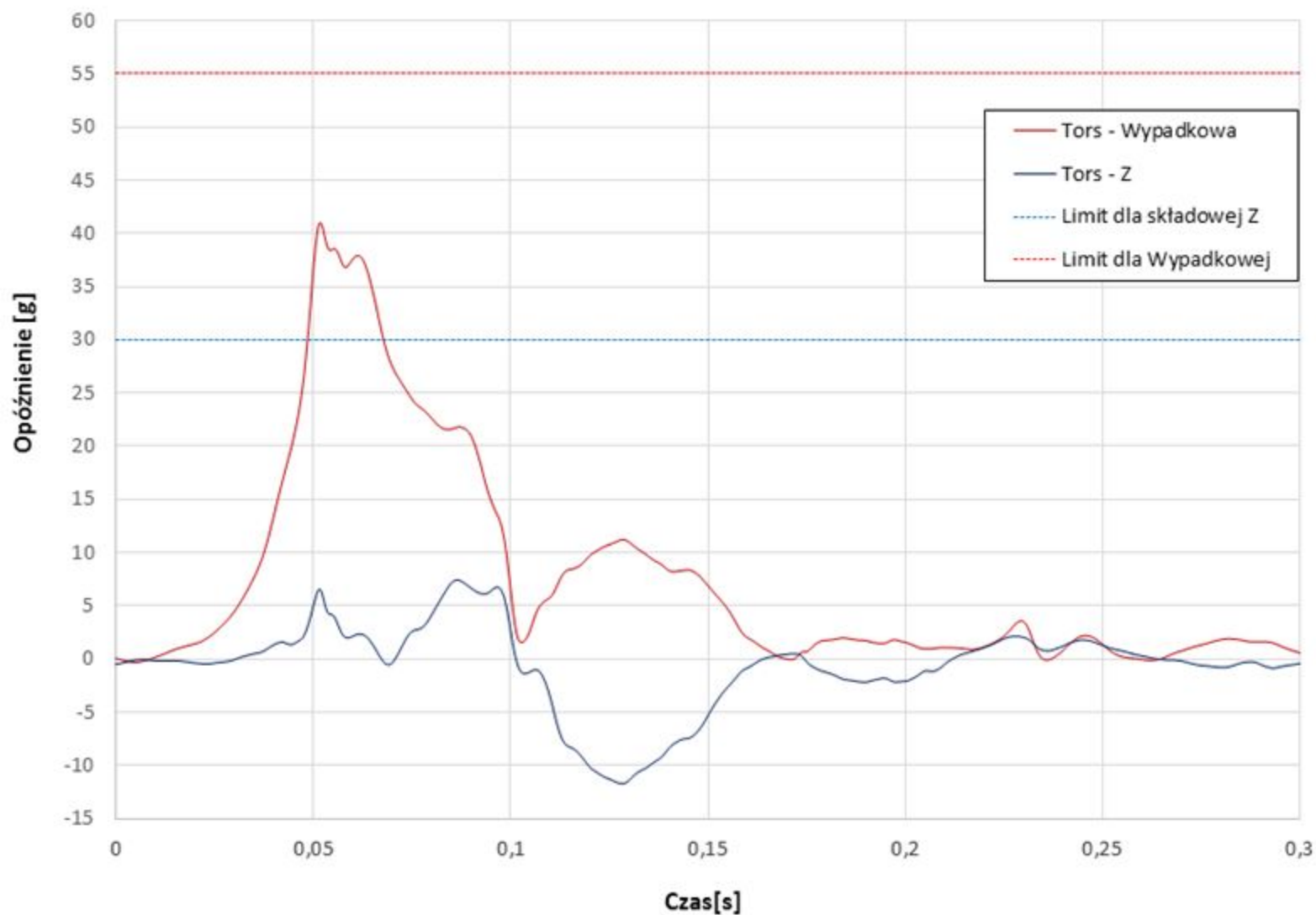
Graph 4. Decelerations of the chest for 32 kg dummy during dynamic test - variant 1
