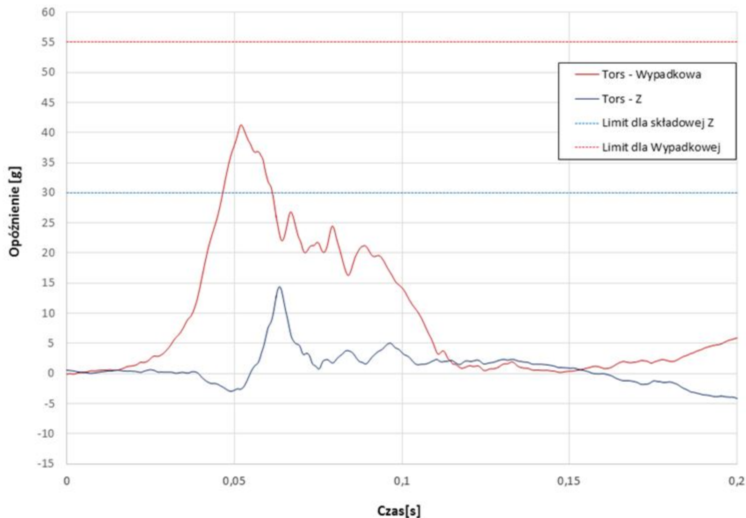
Graph 3. Decelerations of the chest for 22 kg dummy during dynamic test - variant 1
